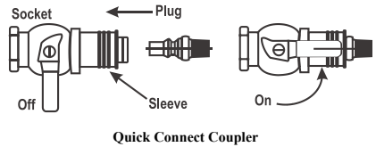
Quick Connect Coupler
